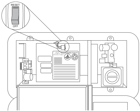
Reset switch located through exterior access
