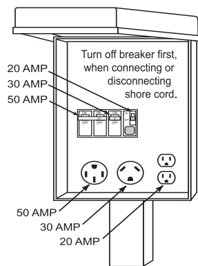
Typical Power Pedestal 020125
