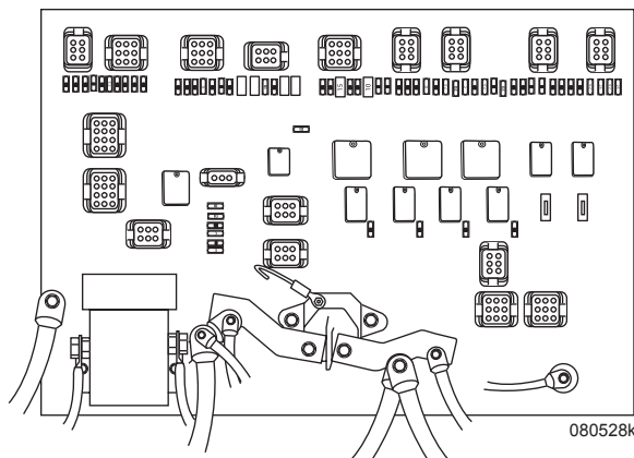
Representation of front distribution panel layout. Components and location will vary with options and changes to motorhome.
