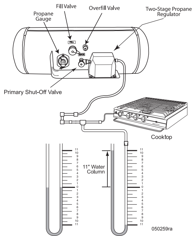
U-Tube Testing Layout
