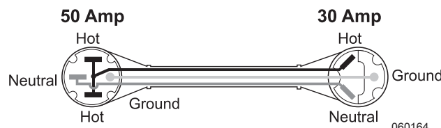
060164 Typical 50-30 Amp Adapter: Adapts 50 Amp Shore Cord to 30 Amp Shore Power Outlet
