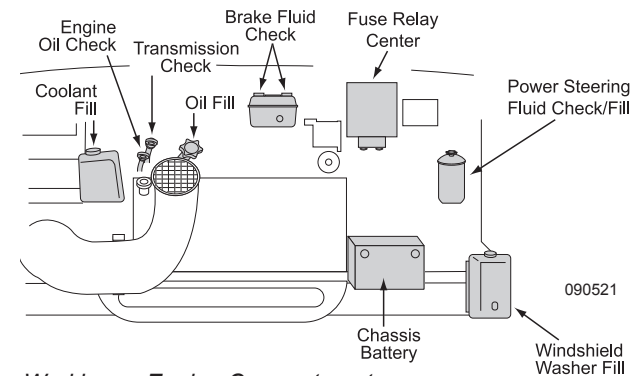
Workhorse Engine Compartment
