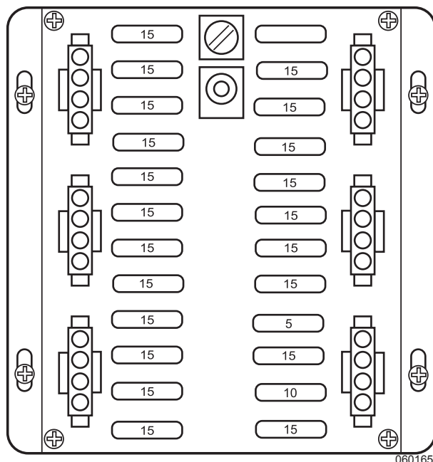
A representation of distribution fuse panel. Actual panel will vary with options and changes to the motorhome.
