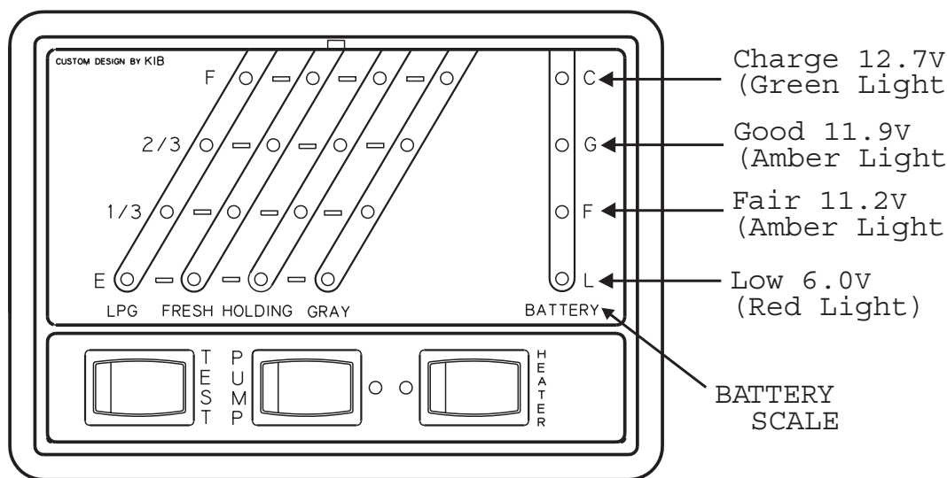
Monitor Panel.
