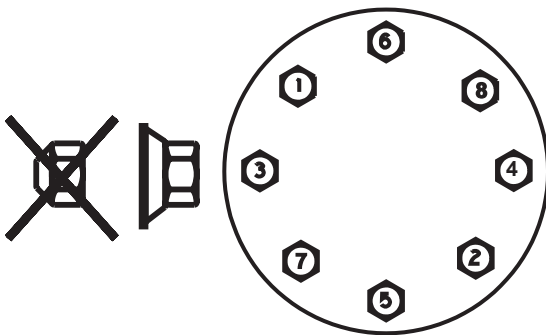
Lug Nut and Sequence
