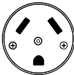
50 AMP Outlet.
